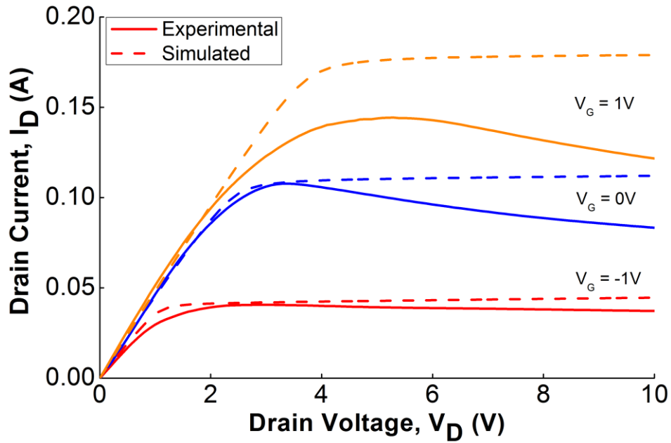
Figure 5.7 Simulated drain current I-V without self-heating effect for an AlGaN/GaN HFET with gate length, L_G = 1\mu\text{m} ; source to drain spacing, L_{SD} \approx 10\mu\text{m} and gate width, W = 200\mu\text{m} obtained from our industrial partners
