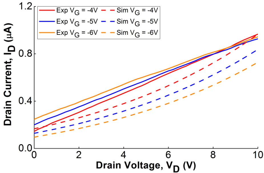
Figure 5.11 Simulated subthreshold current versus experimental subthreshold current for an AlGaIn/GaN HFET with gate length, L_G = 1\mu\text{m} ; source to drain spacing, L_{SD} \approx 5\mu\text{m} and gate width, W = 100\mu\text{m} obtained from our industrial partners
