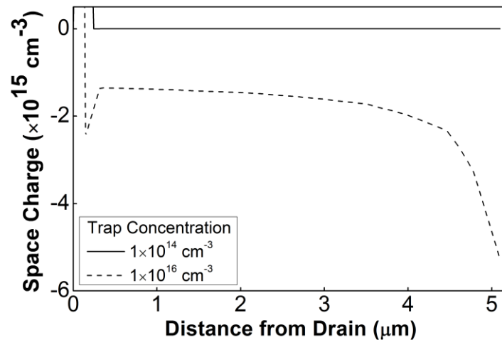
Figure 4.37 Space charge profile at 600V for acceptor concentration N_T = 10^{14} \text{ cm}^{-3} and 10^{16} \text{ cm}^{-3} , barrier height is 0.4eV and bulk doping N_D = 10^{14} \text{ cm}^{-3}
