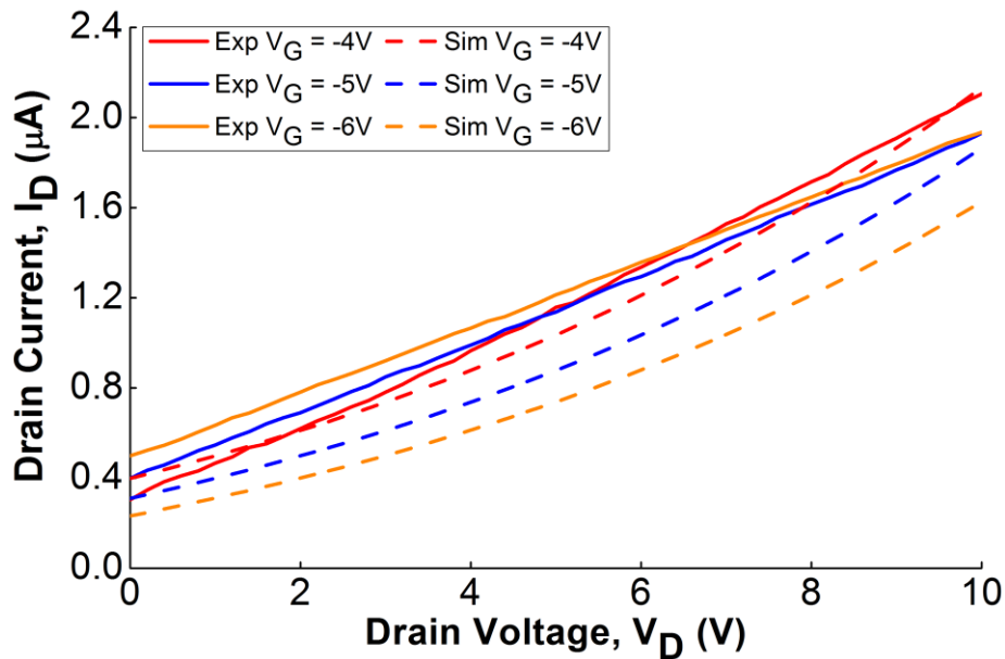
Figure 5.12 Simulated subthreshold current versus experimental subthreshold current for an AlGaIn/GaN HFET on sapphire substrate with gate length, L_G = 1\mu\text{m} ; source to drain spacing, L_{SD} \approx 5\mu\text{m} and gate width, W = 50\mu\text{m} obtained from our industrial partners
